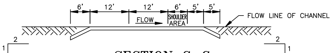
SECTION C-C
