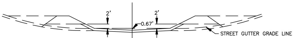
SECTION F-F
